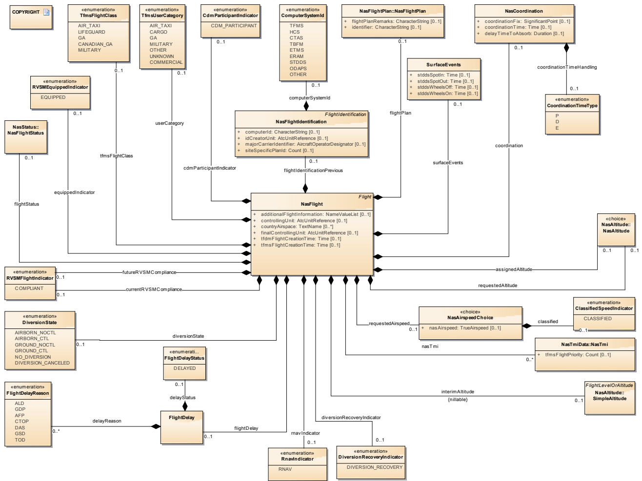
Figure 9: NasFlightData
