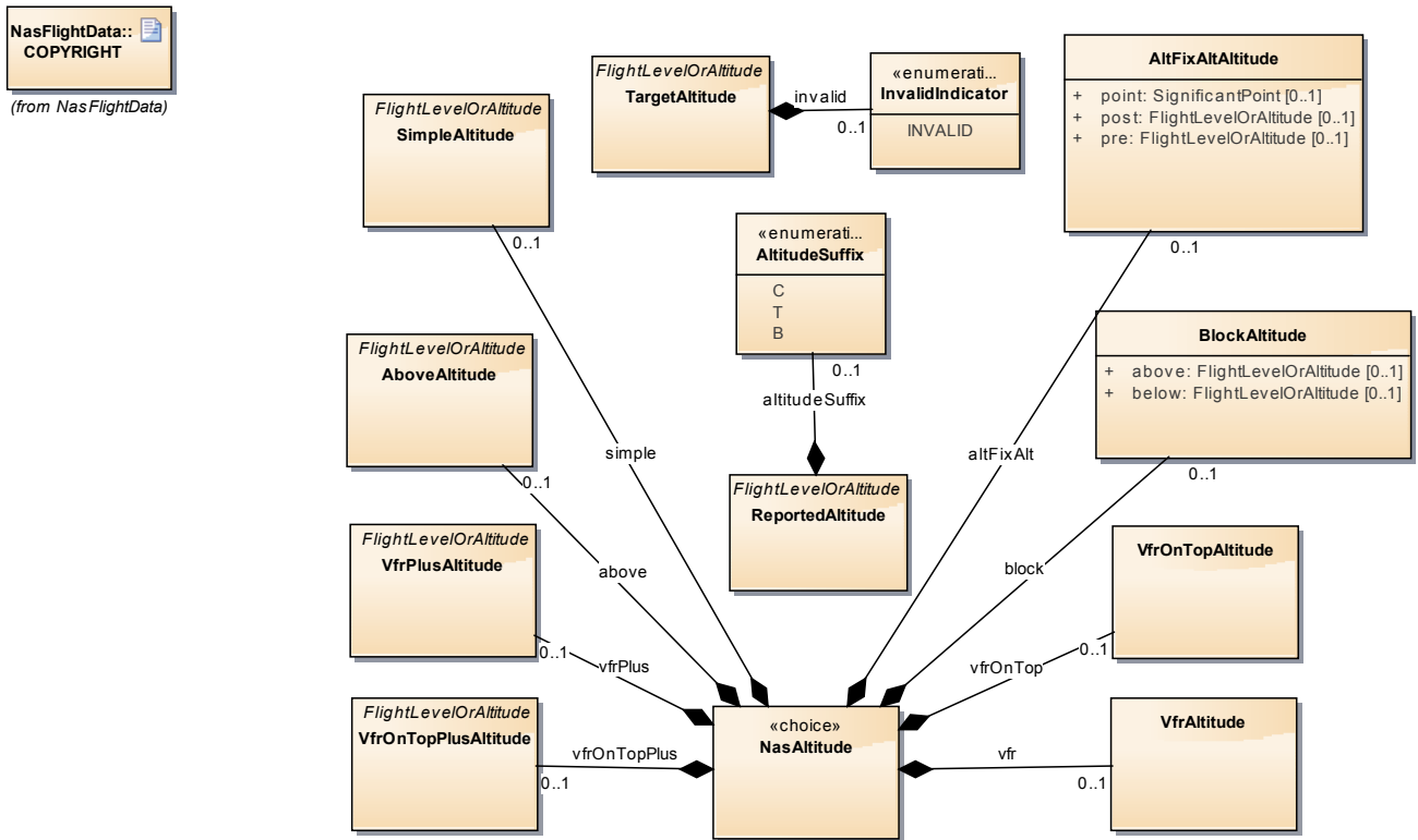
Figure 3: NasAltitude
