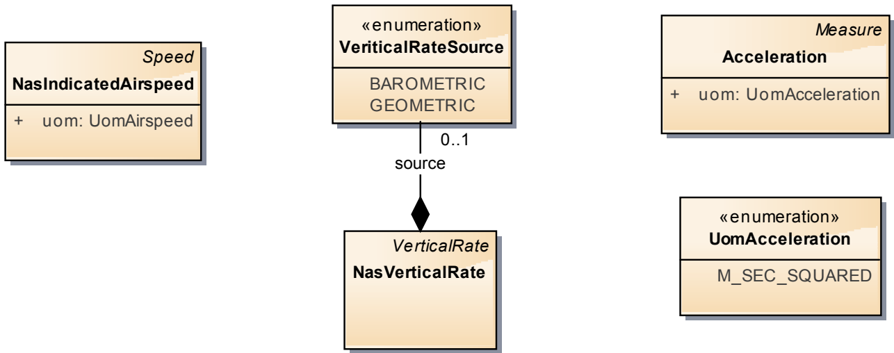
Figure 12: NasMeasures
