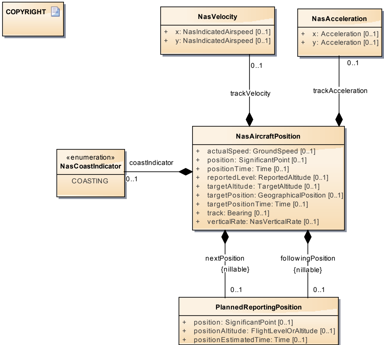
Figure 14: NasPosition
