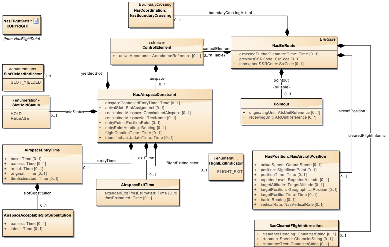
Figure 8: NasEnRouteData
