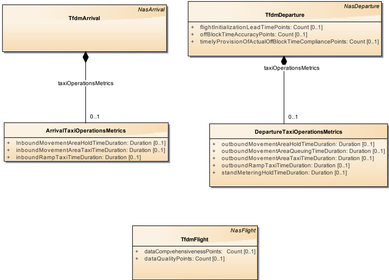
Figure 17: NasTfdm
