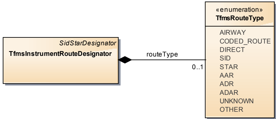
Figure 2: NasAirspace
