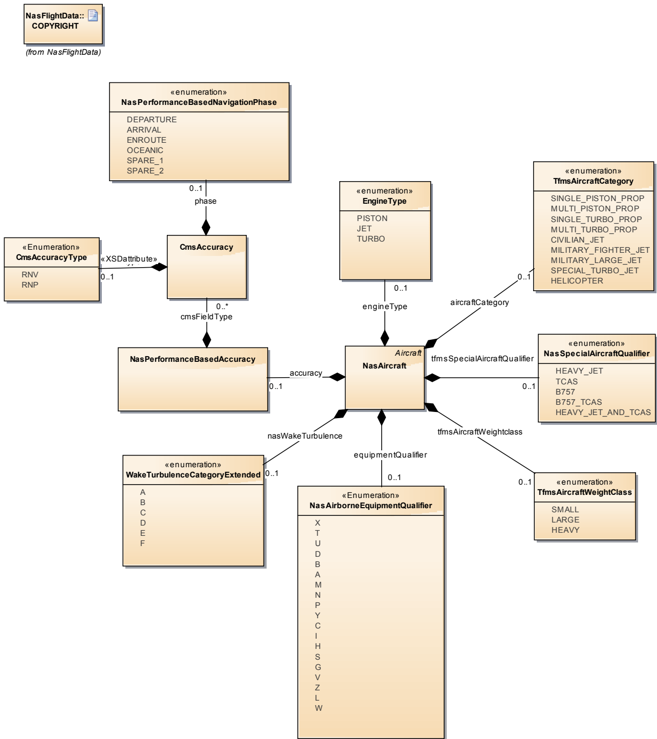
Figure 1: NasAircraft
