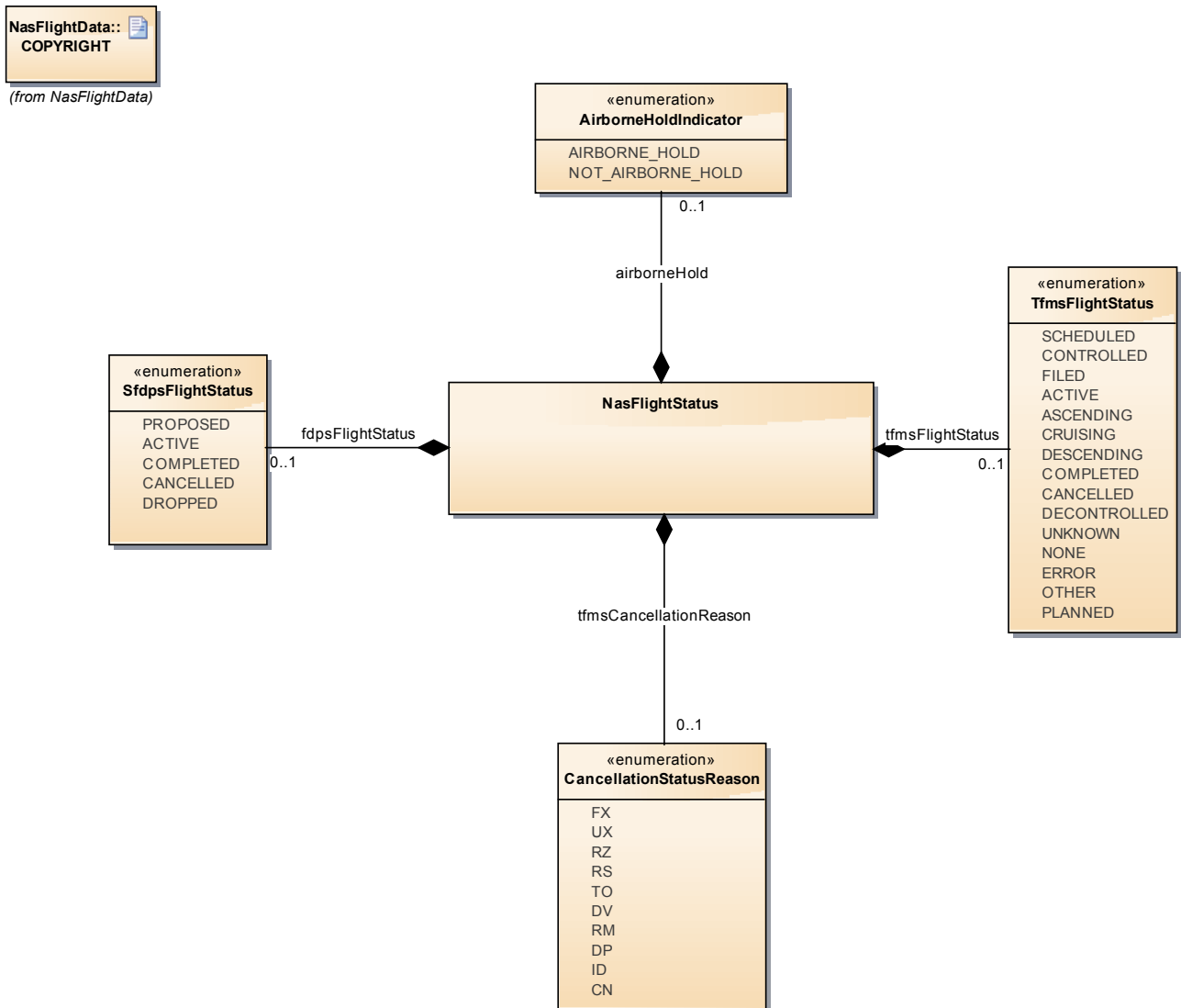
Figure 15: NasStatus
