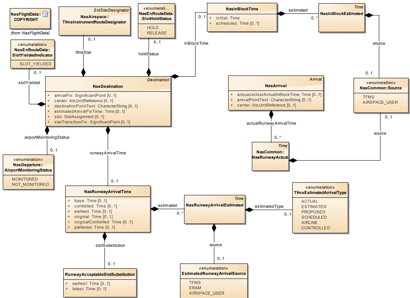
Figure 4: NasArrival
