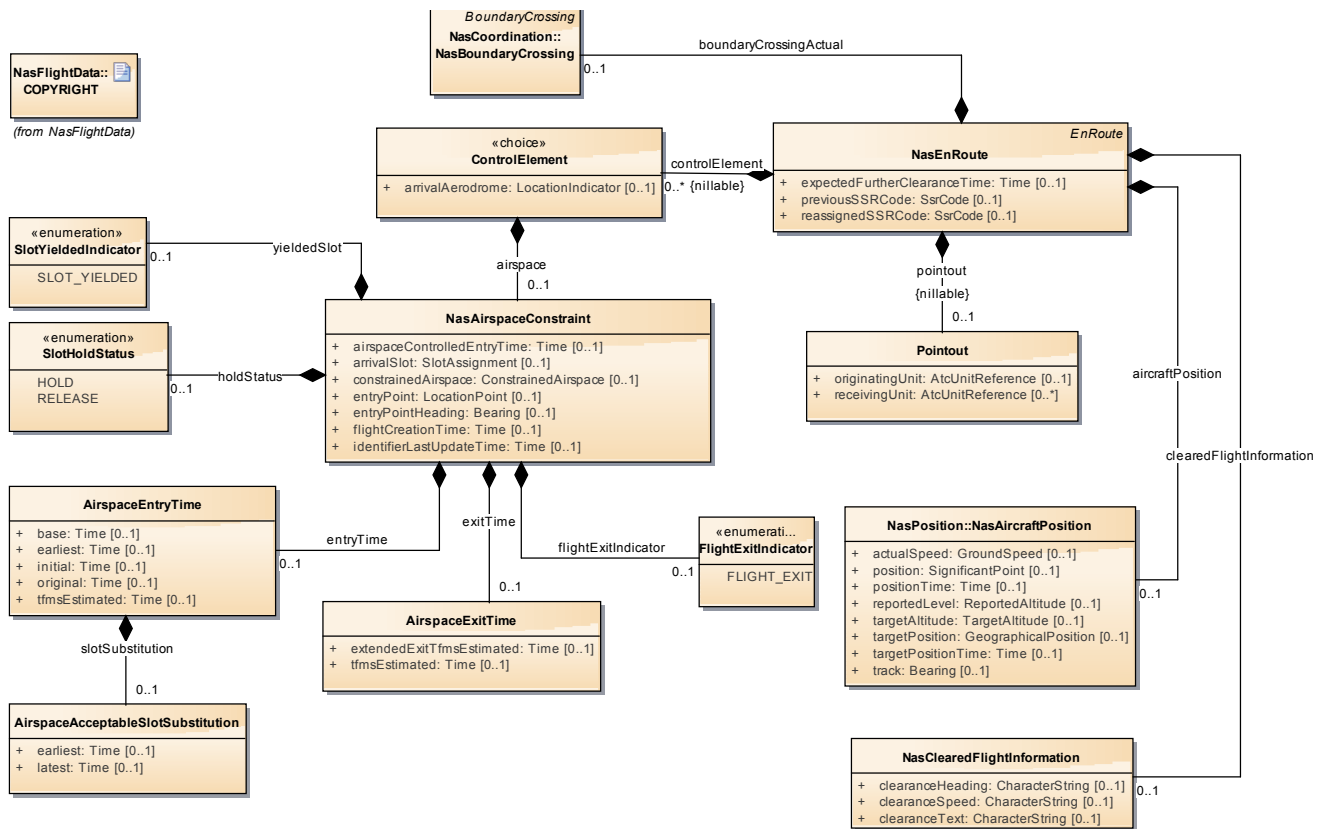
Figure 8: NasEnRouteData
