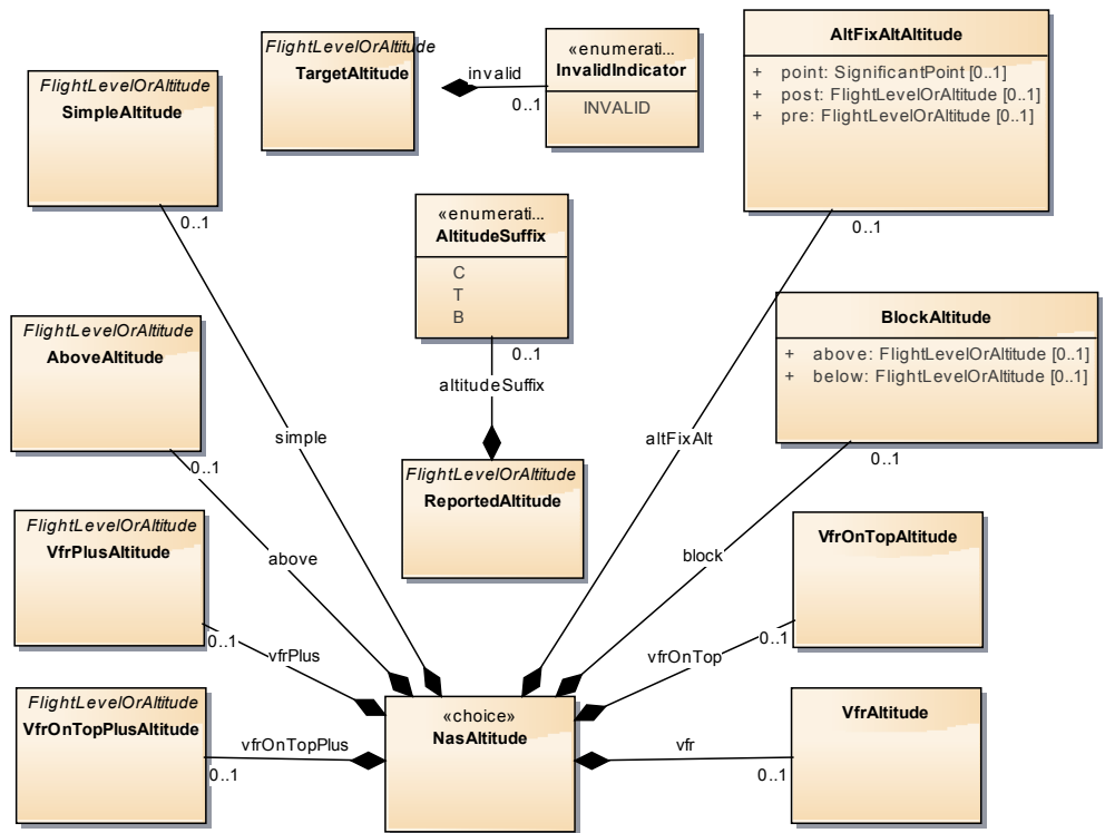
Figure 3: NasAltitude
