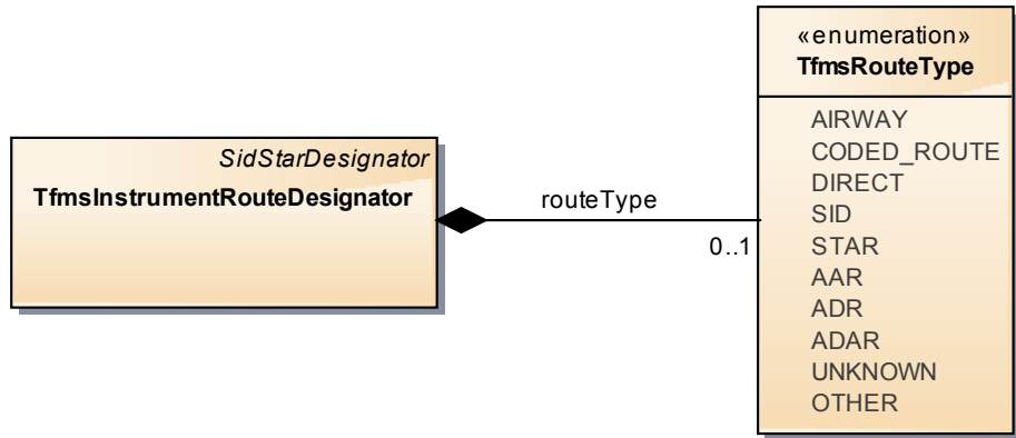
Figure 2: NasAirspace
