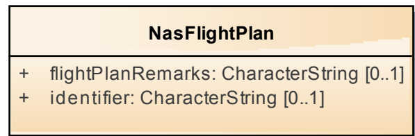
Figure 11: NasFlightPlan
