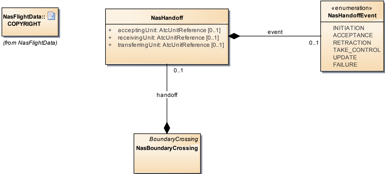
Figure 6: NasCoordination
