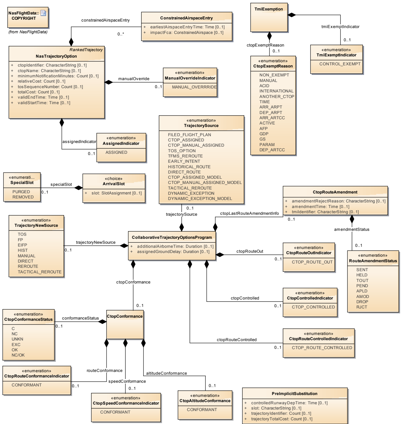
Figure 18: NasTrajectoryOptions
