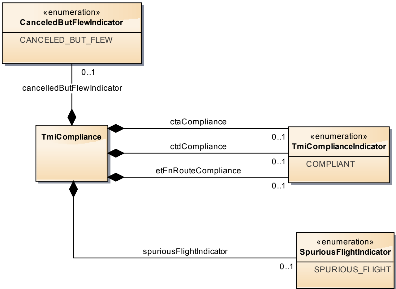
Figure 16: NasTmiCompliance
