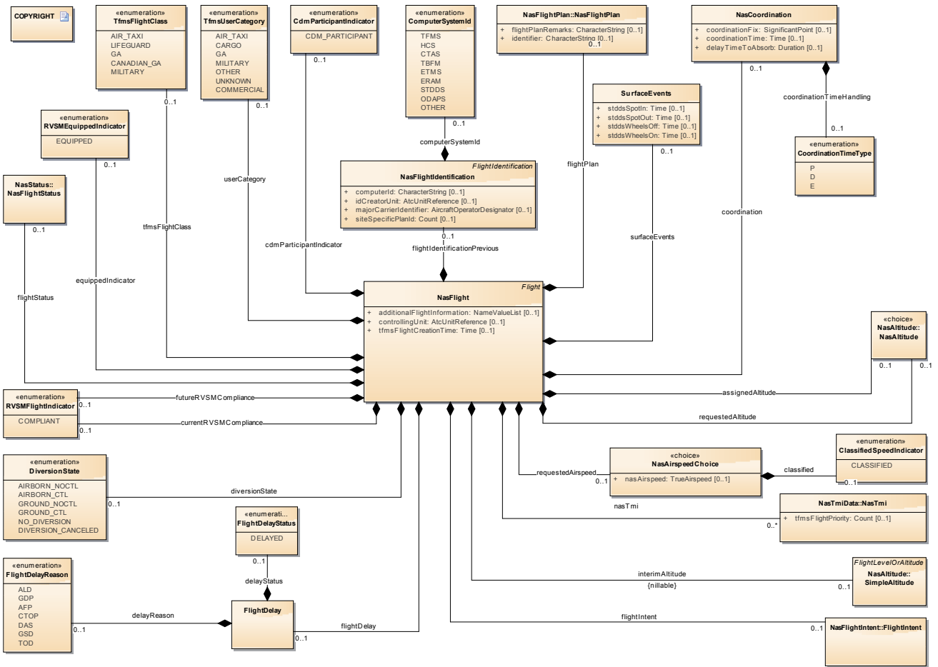
Figure 9: NasFlightData
