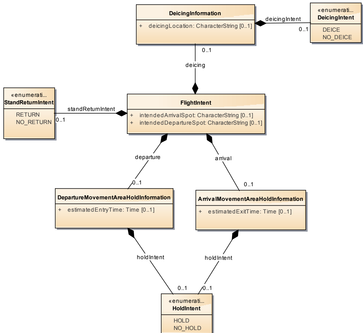
Figure 10: NasFlightIntent
