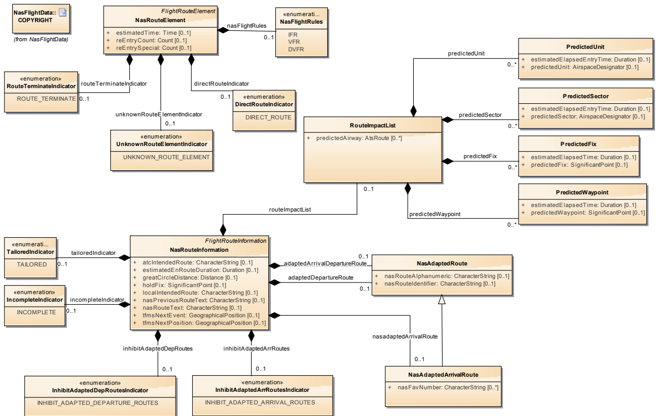
Figure 14: NasRoute
