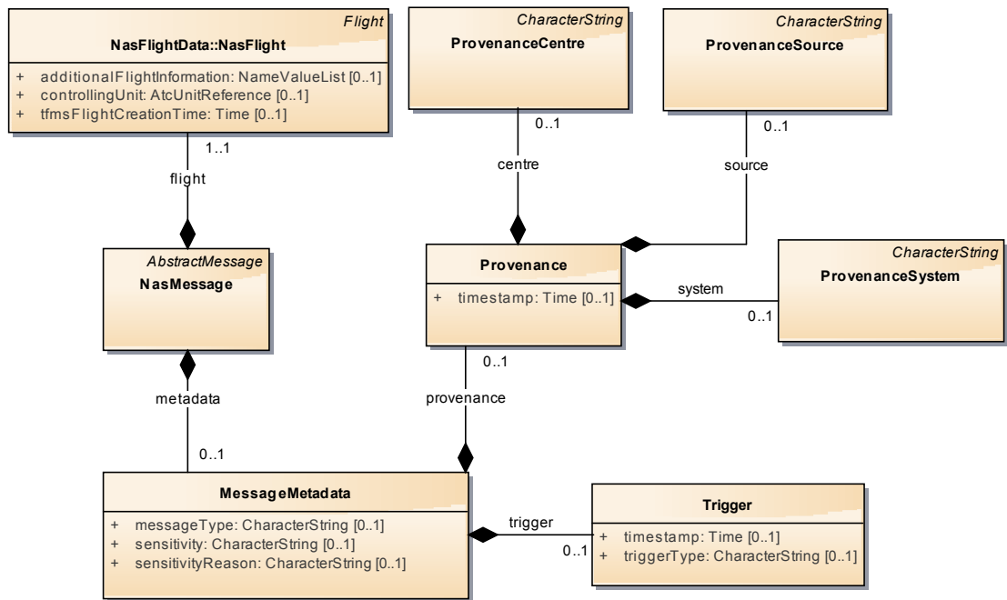
Figure 12: NasMessage
