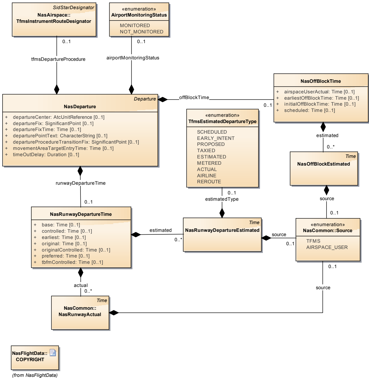
Figure 7: NasDeparture
