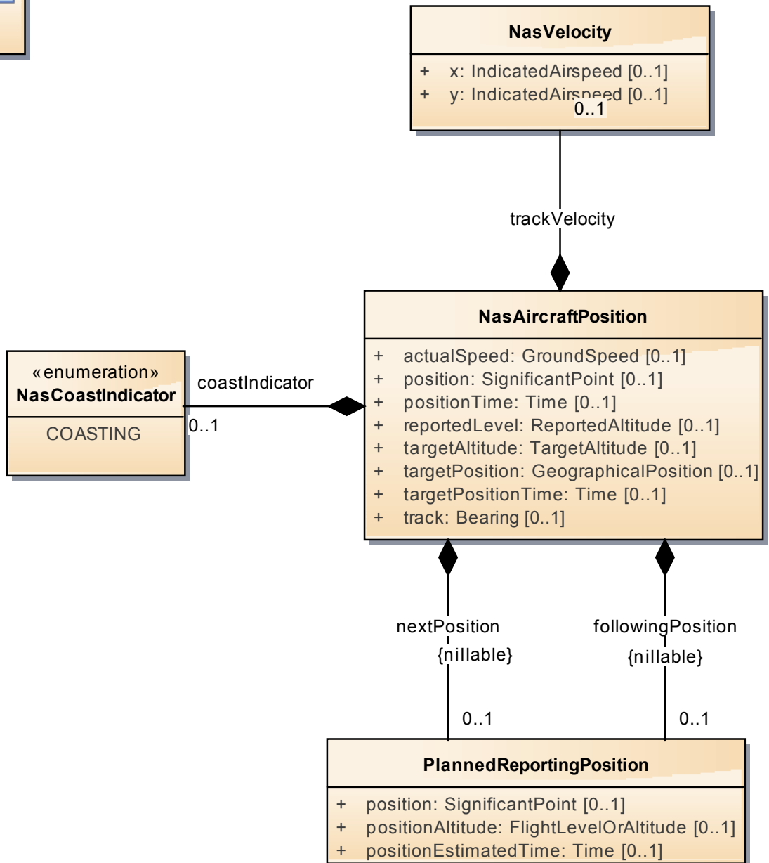
Figure 13: NasPosition
